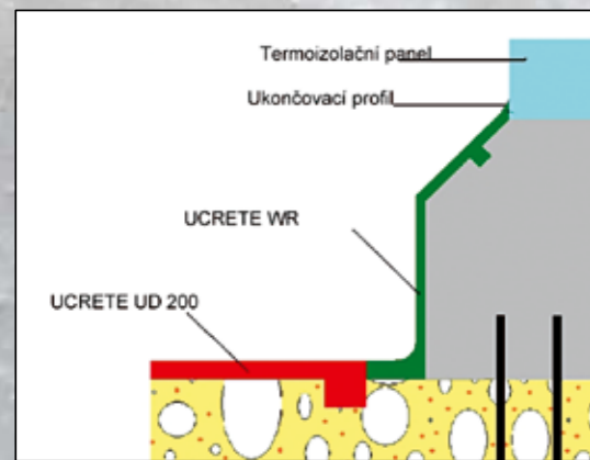
Obr. 4 Detail u zidky
